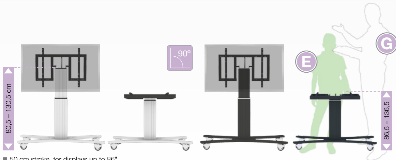
Image shows: SCETTAC with Clevertouch Plus display
